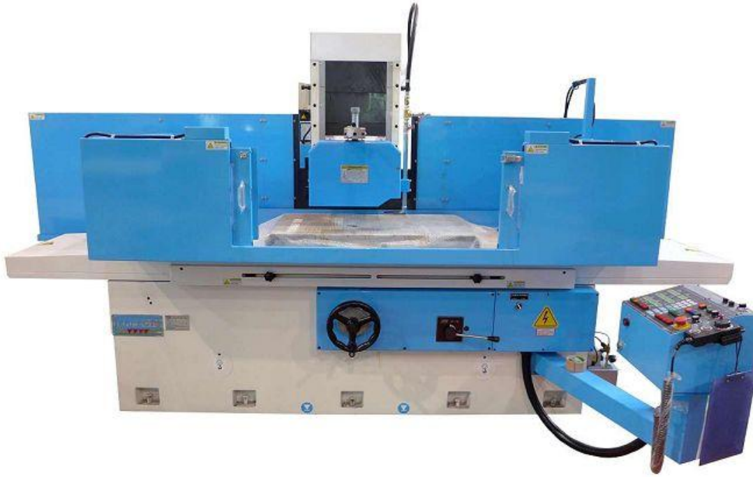
Grinder with 600x1000mm +back water splash shield+semi enclosed splash shield
